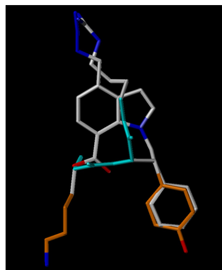
Figure 2. Overlay of the crystal structure of 7 with the K22–Y23–R24 residues from ShK.
